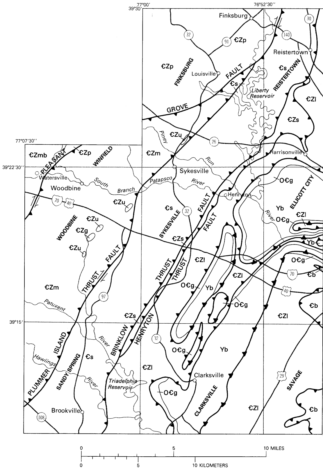
Figure A2. Generalized geologic map of part of the Maryland Piedmont. Intrusive rocks not shown. Geology of the Reisterstown quadrangle modified from Crowley (1977); geology of the Finksburg quadrangle modified from Muller and others (1989); geology of the Ellicott City quadrangle modified from
