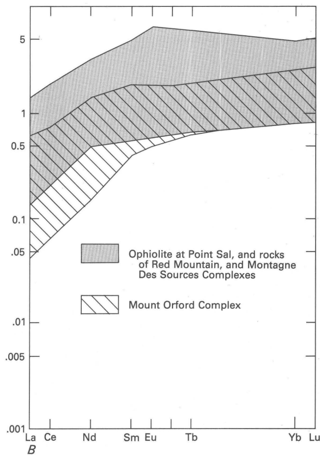
Figure A6. Chondrite-normalized plots comparing pyroxenite of the Soldiers Delight Ultramafite (Sy-H-5-2) with other ultramafic rocks
