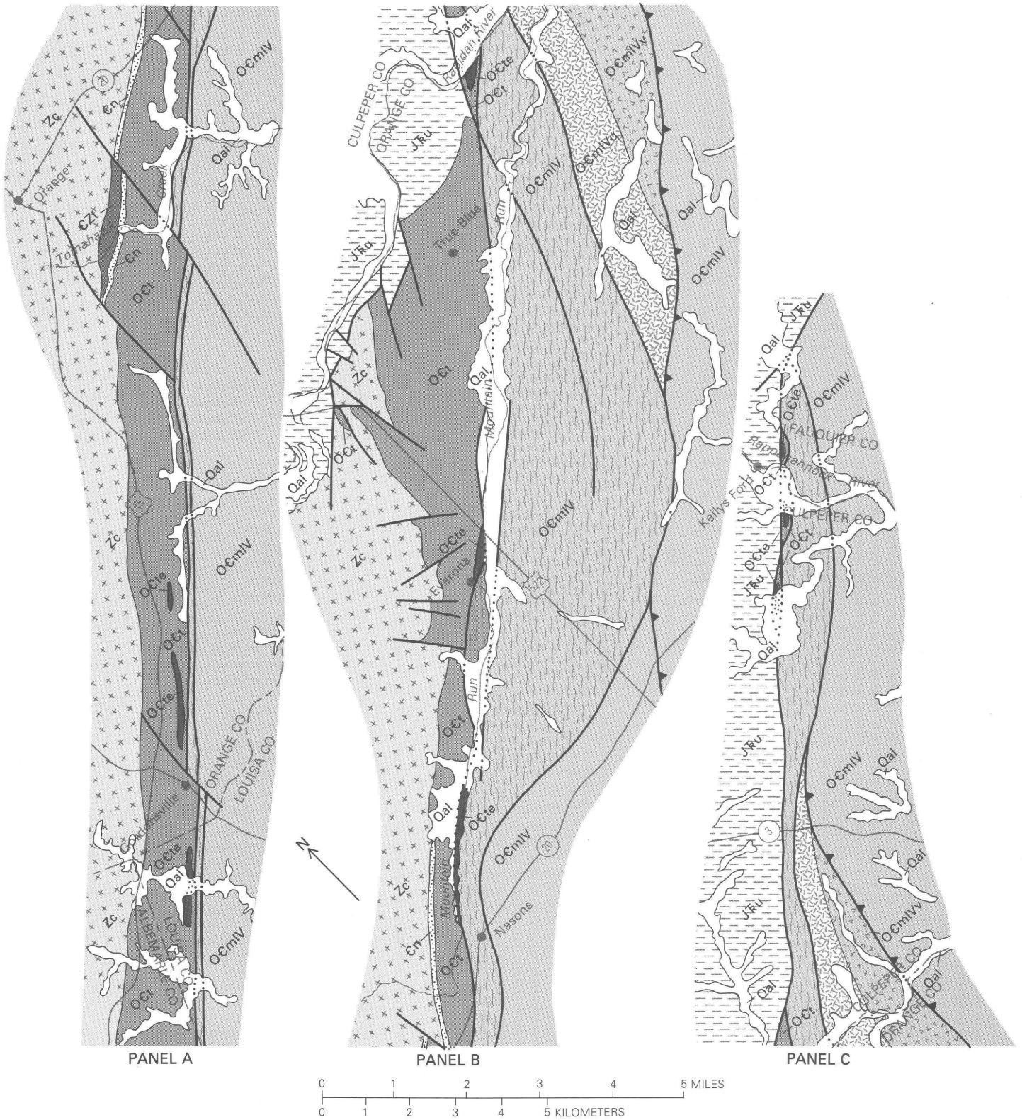
Figure B1. Generalized geologic map showing a part of the western Piedmont and eastern Blue Ridge provinces, north-central Virginia.
