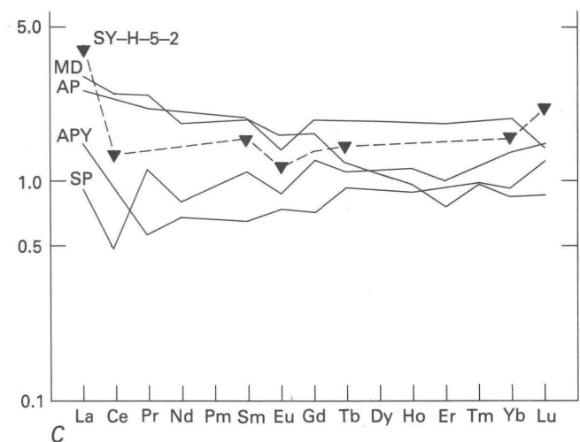
Figure A6. Chondrite-normalized plots comparing pyroxenite of the Soldiers Delight Ultramafite (Sy-H-5-2) with other ultramafic rocks
