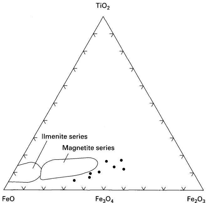
Figure 4.4. \text{TiO}_2 - \text{FeO} - \text{Fe}_2\text{O}_3 (mole percent) diagram for samples (solid circles) from the Dalecarlia Intrusive Suite showing their oxidation state. Magnetite and ilmenite series fields from Jin and others (1981).
