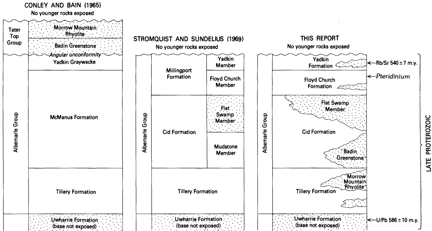
FIGURE 1.—Comparison of stratigraphic nomenclature proposed in this report with that of Conley and Bain (1965) and of Stromquist and Sundelius (1969). Approximate levels of fossils and radiometric dates and inferred ages are shown at right. Volcanic units indicated diagrammatically by pattern.
