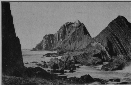
PLATE I.—STEEPLY TILTED ROCKS OF SAN PEDRO POINT, SAN MATEO QUADRANGLE. Shales and sandstones of Martinez formation.
