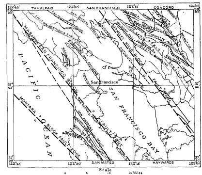
FIGURE 2.—Outline map of the Tamalpais, San Francisco, Concord, San Mateo, and Haywards quadrangles, showing the limits of the great fault blocks, the larger faults, and the areas of folds.
