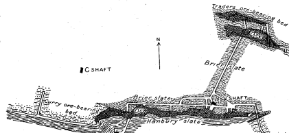
Fig. 9.—Horizontal section of the West Vulcan mine at the eighth level. Scale: 1 inch = 250 feet.
