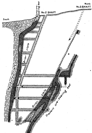
Fig. 10.—Vertical north-south cross section of the West Vulcan mine. Scale: 1 inch = 250 feet.
