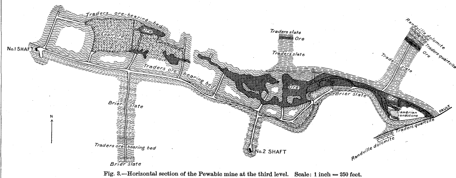
Fig. 3.—Horizontal section of the Pewabic mine at the third level. Scale: 1 inch = 250 feet.
