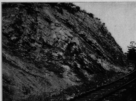
PLATE VII.—VIEW IN LOUISVILLE AND NASHVILLE RAILROAD CUT IN LONE PINE GAP, AT BIRMINGHAM. Looking east. Fort Payne chert (at right), Chattanooga shale (dark streak near middle), and probably Frog Mountain sandstone below, resting unconformably upon Clinton shale (at the extreme left).
