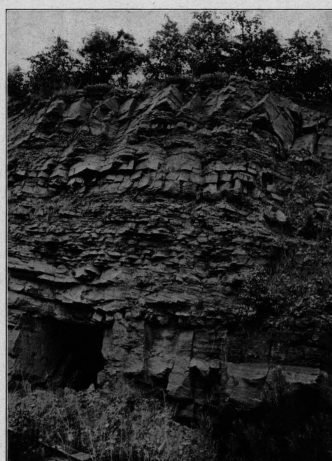
PLATE V.—FERRUGINOUS SANDSTONE AND SHALE OF THE CLINTON FORMATION OVERLYING THE BIG SEAM OF IRON ORE AT SPAULDING. Looking east.
