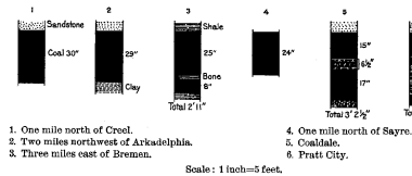
FIGURE 9.—Sections of the Black Creek coal.
