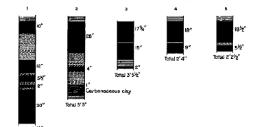
FIGURE 13.—Sections of Newcastle and Nickel Plate coals.
