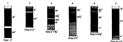
FIGURE 15.—Sections of Pratt coal.
