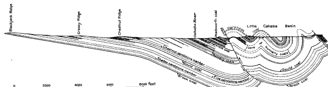
FIGURE 17.—Cross section of the Cahaba coal field, showing structure and repetition of the Harkness coal.
