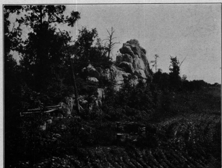
PLATE X.—DIKELIKE OUTCROP OF VERTICAL HARTSELLE SANDSTONE MEMBER 1 1/2 MILES EAST OF NEWCASTLE. Looking north. This feature extends north to Pinson and is called Rocky Row.
