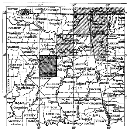
FIGURE 1.—Index map of northeastern Alabama and northwestern Georgia. Darker ruled area covered by Birmingham folio. Other published folios indicated by lighter ruling, as follows: Nos. 2, Ringgold; 6, Chattanooga; 8, Seawaco; 19, Stevenson; 20, Cleveland; 25, Gadsden; 78, Rome.
