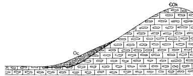
FIGURE 3.—Ideal section half a mile west of Chalkville. Shows unconformable contact of Chickamauga limestone (Oc) with the underlying Knox dolomite (Ck). Vertical scale twice the horizontal.
