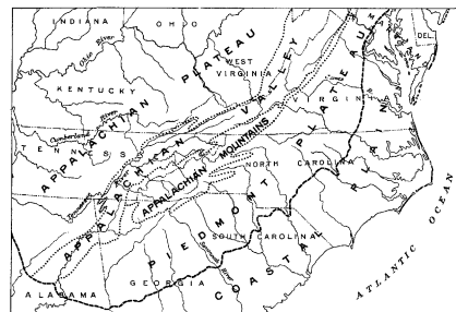
FIGURE 2.—Map of the southern part of the Appalachian province, showing its physiographic divisions and its relation to the Coastal Plain.
