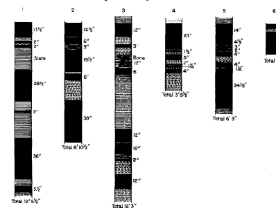
FIGURE 12.—Sections of Mary Lee coal.
