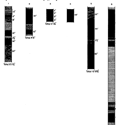
FIGURE 16.—Sections of Harkness, Wadsworth, and Mammoth coals.
