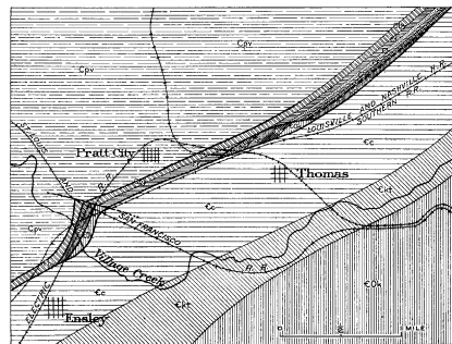
FIGURE 8.—Map of faulted areas in the vicinity of Pratt City and Thomas. Cpv, Pottsville formation; Cby, Boyle sandstone member; Cf, Floyd shale; Ch, Hartselle sandstone member; Cfr, Fort Payne chert; Cd, Chattanooga shale and Frog Mountain sandstone; Cs, Clinton formation; Cc, Conasauga limestone; Ck, Knox dolomite; Ckt, Kenton dolomite member; Cc, Conasauga limestone.
