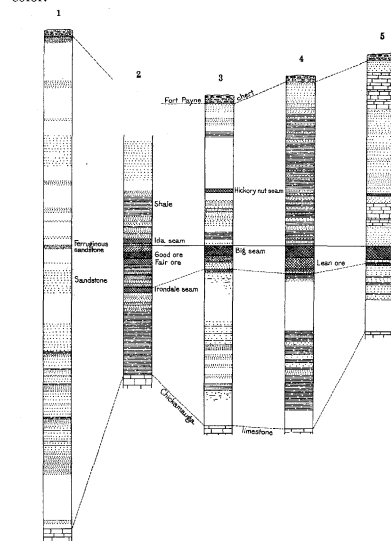
FIGURE 5.—Sections of Clinton formation showing variation in thickness and character of the rocks.
