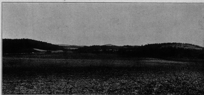
PLATE III.—CHARACTERISTIC HILLY TOPOGRAPHY OF THE KNOX DOLOMITE AREAS. Crest of Red Mountain, composed of the Clinton formation, in the distance. Looking east from highway about 1 mile south of Pinson.
