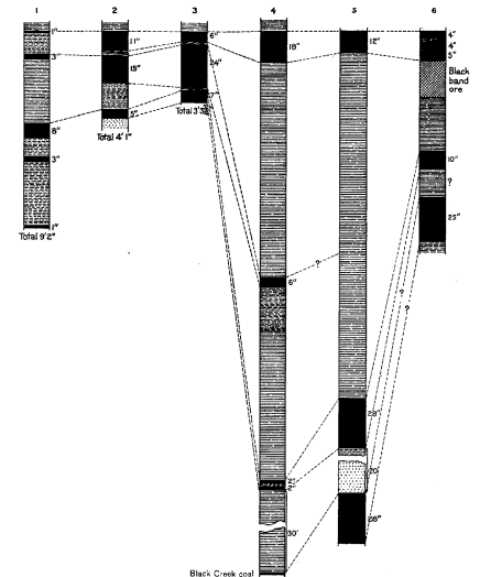
FIGURE 10.—Sections of the Jefferson coal.
