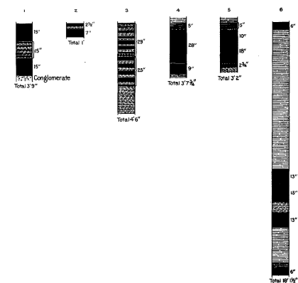
FIGURE 11.—Sections of Jagger and Blue Creek coals.
