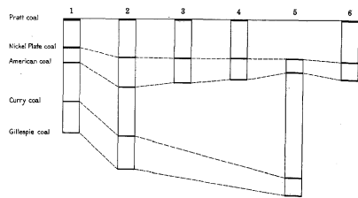
FIGURE 14.—Sections showing relations of the Nickel Plate and American coals.
