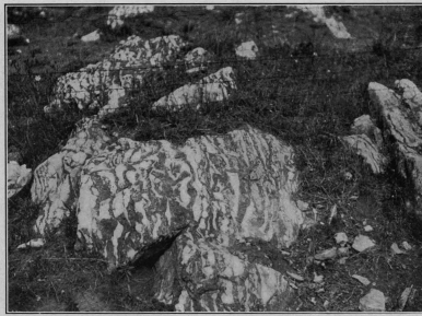
FIGURE 16.—IRREGULAR ARGILLACEOUS AND SILICEOUS BANDING IN THE LOWER BEDS OF THE BEEKMANTOWN LIMESTONE, 1 MILE SOUTHWEST OF AQUA.
