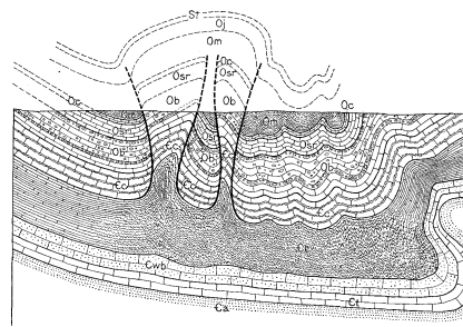
FIGURE 4.—Cross section of Mercersburg anticline along the line E-E on the Mercersburg areal geology map; reduced one-fourth.
