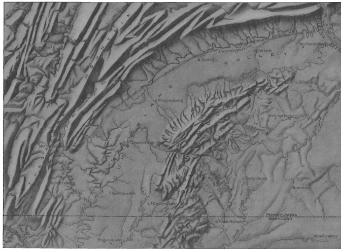
FIGURE 2.—Relief map of Cumberland Valley, the Appalachian Valley ridges (on the left), and South Mountain (on the right), in southern Pennsylvania. The eastward curving of the valley and bounding ridges toward the northeast is clearly shown; also the offset of the west face of South Mountain into the valley opposite Waynesboro and Chambersburg. The doubling back of the ridges northwest of the valley is due to folding of the hard strata. The Mercersburg and Chambersburg quadrangles extend from McConnellsburg to the mountain front east of Chambersburg, and southward to Waynesboro. Scale, 1 inch = 10 miles.
