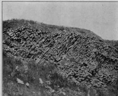
FIGURE 10.—CHARACTERISTIC THIN-BEDDED LIMESTONE OF THE CHAMBERSBURG FORMATION, IN RAILROAD CUT 2 MILES SOUTHWEST OF MARION.
