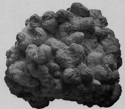
FIGURE 14.—"CAULIFLOWER" CHERT FROM THE UPPER PART OF THE BEEKMANTOWN LIMESTONE IN THE MERCERSBURG QUADRANGLE.
