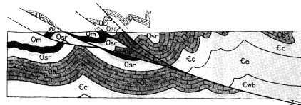
FIGURE 3.—Cross section of the Greencastle faults, illustrating progressive movement along successive fault planes.
