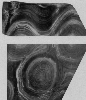
FIGURE 13.—CRYPTOZOON PROLIFERUM FROM LOWER PART OF THE CONOCOCHEAQUE FORMATION, 2 MILES WEST OF FAYETTEVILLE. Natural size. Upper figure, cross section; lower figure, under side of same specimen.
