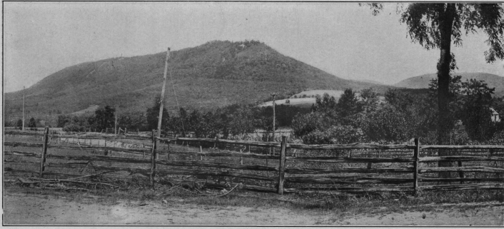
FIGURE 7.—JORDAN KNOB SYNCLINAL MOUNTAIN, FROM FORT LOUDON. The western limb of the syncline is shown terminating in Jordan Knob in the center of the picture. The crest of the mountain is composed of Tuscarora sandstone; the cleared fields on the slope are of Martinsburg shale.
