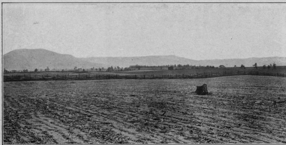
FIGURE 12.—SCHOOLEY PENEPLAIN PRESERVED ON CROSS MOUNTAIN. The level-topped ridge in the middle distance is Cross Mountain. At the right is the lower ridge of Cove Mountain, and at the left is Two Top Mountain. The foreground represents the Somerville peneplain preserved on Martinsburg shale.
