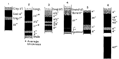
FIGURE 7.—Sections of Helena, Montevallo, and Maylene coal beds 1. Helena coal in Savage Creek mine 2. Helena coal in Superior mine 3. Montevallo coal in SW ¼ sec. 18, T. 22 S., R. 4 W. 4. Montevallo coal in Aldrich mine, ninth west heading, near main slope 5. Montevallo coal in Aldrich mine, room 27 off west heading 6. Maylene coal in Clinch mine, face of fourteenth west heading
