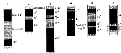
FIGURE 4.—Sections of Gould, Nunnally, Big Bone, and Buck coal beds. 1. Gould (G) coal at Old Peter mine, in NE. \frac{1}{4} sec. 12, T. 24 N., R. 11 E. 2. Nunnally coal, next to top bed (Cubical), in NE. \frac{1}{4} sec. 12, T. 24 N., R. 11 E. (estimated). 3. Nunnally coal, top bed (Figh), in NE. \frac{1}{4} sec. 12, T. 24 N., R. 11 E. (estimated). 4. Coke Oven (Big Bone) coal on Southern Railway in SE. \frac{1}{4} sec. 9, T. 20 S., R. 4 W. 5. Buck (Atkins) coal on Louisville & Nashville Railroad at Pine Woods. 6. Buck (Atkins) coal on Southern Railway in NE. \frac{1}{4} sec. 20, T. 21 S., R. 4 W.
