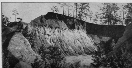
PLATE 11.—SHELBY IRON ORE DIGGINGS At top there is 15 feet of red loam carrying best quality of lump ore, underlain by light-colored sand and quartz gravel, possibly of Cretaceous age.
