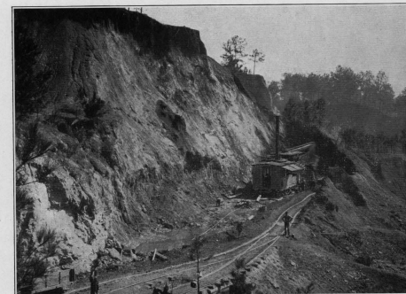
PLATE 15.—IRON ORE DIGGINGS AT SHELBY Ore is in pockets in decayed rock, which is reported to extend nearly 100 feet below the bottom of the pit. The clay seems to fill an ancient sink hole.
