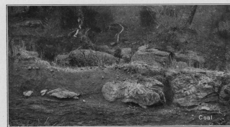
PLATE 12.—CONASAUGA LIMESTONE OVERTHRUST ON A COAL BED IN THE POTTSVILLE FORMATION Shoal Creek, 1.5 miles southwest of Aldrich, in the Cahaba coal field.
