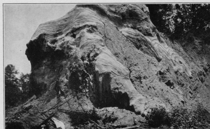
PLATE 14.—RESIDUAL PINNACLE OF CONTORTED NEWALA LIMESTONE EXPOSED IN ORE BANK AT SHELBY
