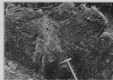
PLATE 6.—BRIERFIELD DOLOMITE INCRUSTED WITH CHARACTERISTIC FRETWORK OF RESIDUAL SILICA Sixmile Creek, about 1 mile northwest of the southwest corner of the Montevallo quadrangle.
