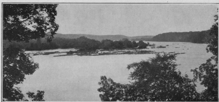
PLATE 1.—COOSA RIVER IN THE SOUTHEAST CORNER OF THE COLUMBIANA QUADRANGLE Looking south from the Narrows. Shows upland surface or old peneplain with intrenched river valley.
