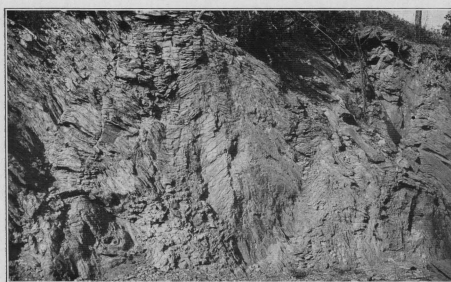
PLATE 5.—CRUMPLED WASH CREEK SLATE 8 MILES SOUTH OF SHELBY
