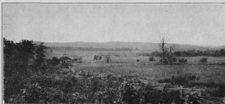
PLATE 2.—VIEW LOOKING NORTHWEST ACROSS SHELBY VALLEY Valley eroded mainly on the Newala limestone. Columbiana Mountain in the distance.
