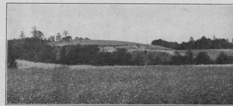
PLATE 3.—ROUNDED HILLS CHARACTERISTIC OF AREAS UNDERLAIN BY WAXAHATCHEE SLATE About 2 miles south of Shelby. Looking east.
