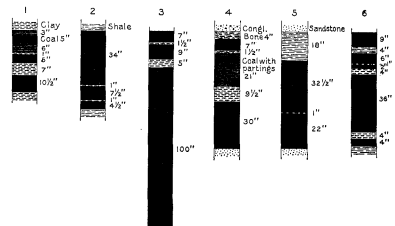
FIGURE 6.—Sections of Gholson and Thompson coal beds 1. Gholson coal at siding to Garnsey mine, Garnsey 2. Gholson coal in Marvel No. 1 mine 3. Gholson coal on Alligator Creek in NE ¼ sec. 7, T. 24 N., R. 11 E. 4. Thompson (upper) coal in Garnsey mine, entrance to ninth west heading 5. Thompson coal in Garnsey mine, face of ninth east heading 6. Thompson coal on Fourmile Creek in the western part of sec. 3, T. 24 N., R. 11 E.
