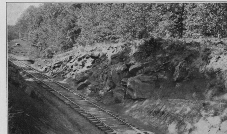
PLATE 9.—FROG MOUNTAIN SANDSTONE (DEVONIAN) LYING ON FOSSILIFEROUS CLAY WHICH IS DECOMPOSED LITTLE OAK LIMESTONE (ORDOVICIAN) Cut on railroad 1 mile northwest of Mosteller, in the eastern part of the Columbiana quadrangle. Between the clay and sandstone is a stratigraphic gap representing the upper part of the Ordovician system, the entire Silurian system, and the lower part of the Devonian system.
