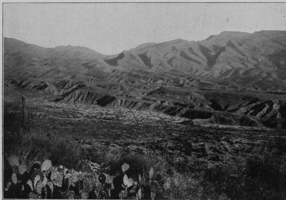
PLATE I.—VIEW LOOKING NORTHEASTWARD ACROSS DRIPPING SPRING VALLEY TO THE MESCAL RANGE. Shows intricately dissected valley fill of Gila conglomerate.
