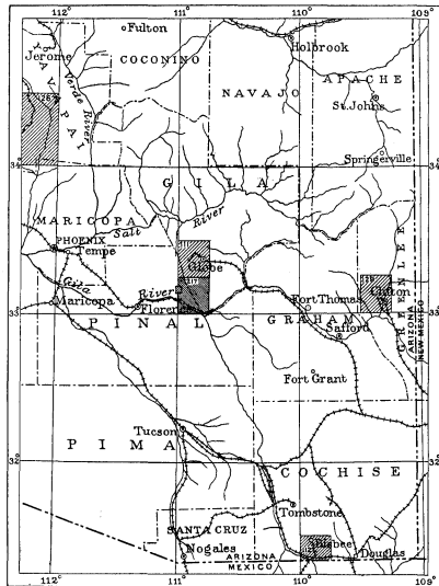
FIGURE 1.—Index map of southeastern Arizona.
