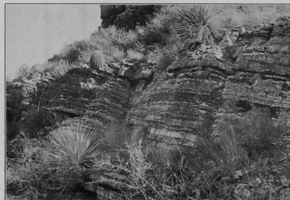
PLATE IV.—TYPICAL HILLSIDE EXPOSURE OF THE CHERTY MESCAL LIMESTONE IN THE DRIPPING SPRING RANGE, 2 MILES SOUTH OF DRIPPING SPRING RANCH.
