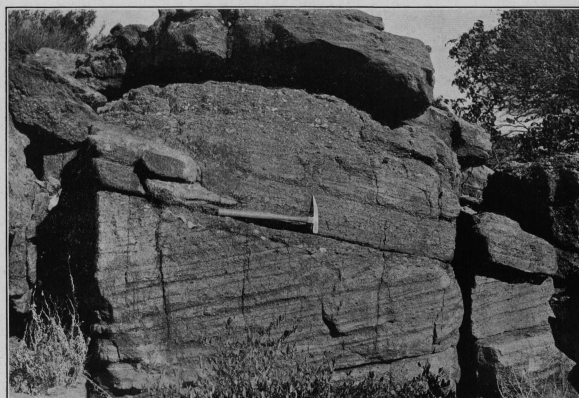
PLATE V.—CROSS-BEDDED PEBBLY TROY QUARTZITE, DRIPPING SPRING RANGE.
