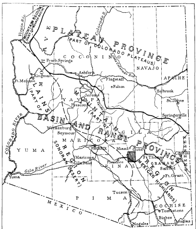
FIGURE 2.—Map of Arizona showing the principal physiographic divisions of the State.
