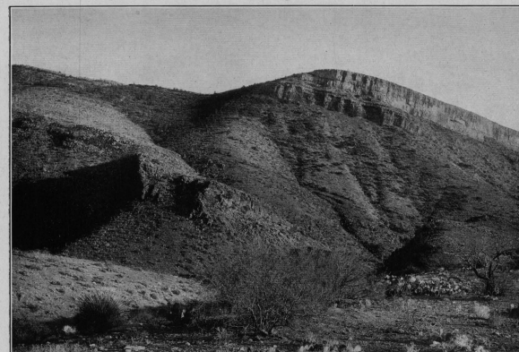
PLATE VI.—TYPICAL HILLSIDE EXPOSURE OF THE DEVONIAN ON EL CAPITAN CREEK, MESCAL RANGE. The Devonian limestone forms the smooth slope between the bluff of Troy quartzite in the middle ground and the cliffs of Tornado limestone above.
