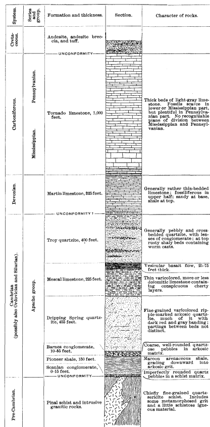
FIGURE 3.—Generalized columnar section of the rocks that crop out in the Ray quadrangle.
