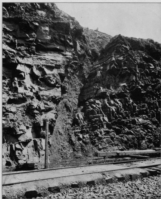
FIG. 31.—FAULT IN SANDSTONE OF NEWARK GROUP, IN RAILROAD CUT WEST OF ARLINGTON, N. J., LOOKING NORTH. Shows broad zone of breccia along the fault plane.
