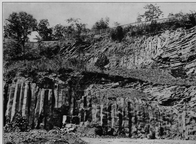
FIG. 30.—BASALT COLUMNS OF FIRST WATCHUNG SHEET, O'ROURKE'S QUARRY, WEST OF ORANGE, N. J. The lower portion of the basalt, which rests on sandstone, presents large vertical columns; the upper portion consists of small radial columns.
