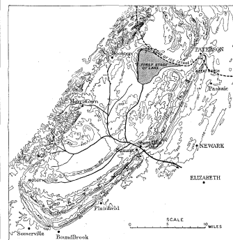
FIG. 16.—An early stage of the glacier during its last invasion, and the initial stage of Lake Passaic. The edge of the ice blocked the Paterson pass across the basalt ridges, and a small lake developed in the basin to the south, which is represented as having an outlet by way of the Short Hills gap across First and Second Watchung mountains.
