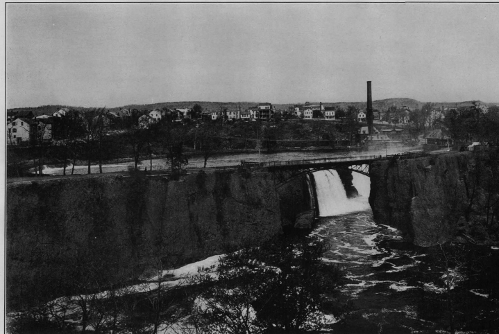
FIG. 28.—GREAT FALLS OF PASSAIC RIVER, PATERSON, N. J. The gorge is cut in Watchung basalt, and the narrow cleft into which the falls have retreated is along the major joint system.
