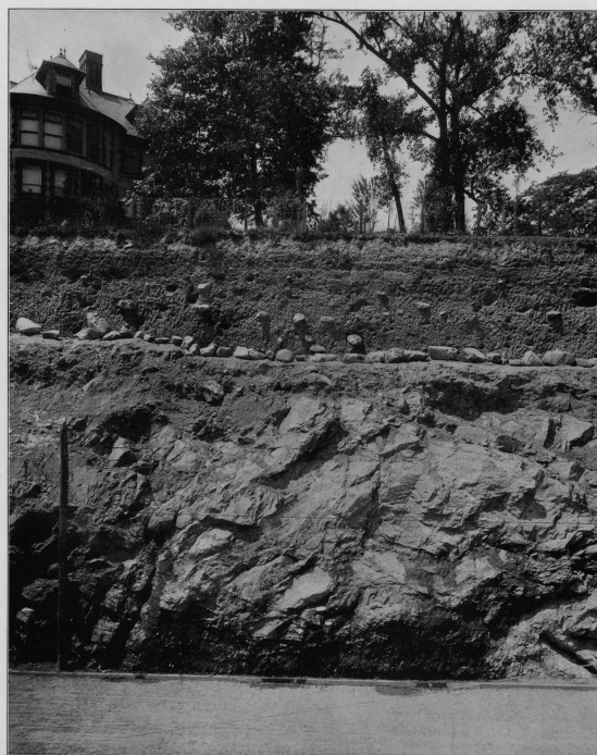
FIG. 32.—SECTION OF GLACIAL TILL ON SERPENTINE, CASTLE POINT, HOBOKEN, N. J.
