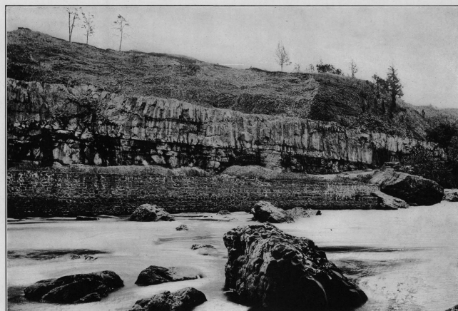
FIG. 29.—CONFORMABLE CONTACT OF BASALT OF THE FIRST WATCHUNG SHEET ON NEWARK SANDSTONE, BELOW FALLS OF THE PASSAIC, PATERSON, N. J. The sandstone forms the base of the section immediately above the retaining wall and is overlain by massive-bedded basalt capped by finely columnar basalt.
