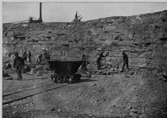
FIG. 13.—CEMENT-ROCK QUARRY IN MILWAUKEE FORMATION AT BERTHELET, JUST NORTH OF MILWAUKEE.
