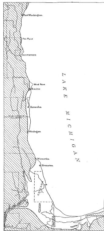
FIG. 8.—Sketch map showing the maximum extent of Lake Chicago, in southeastern Wisconsin, Illinois, and northern Indiana.
