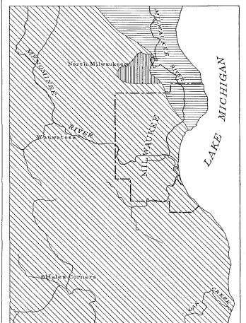
FIG. 2.—Sketch map of Paleozoic formations of the Milwaukee district. Racine limestone (Niagara). Washburn formation (Cayuga). Milwaukee formation (Hamilton). Red rock heavily covered by drift and only occasionally exposed.
