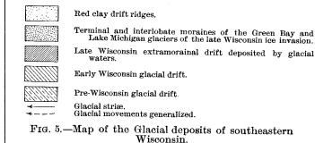
FIG. 5.—Map of the glacial deposits of southeastern Wisconsin.
