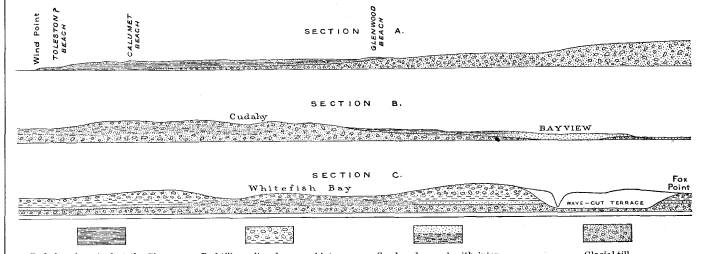
FIG. 7.—Sections exposed in the lake bluff in the Milwaukee Special quadrangle and vicinity. Horizontal scale, 1 inch = 1 mile; vertical scale, 1 inch = 500 feet.
