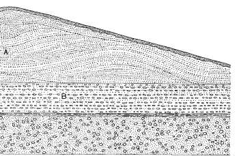
FIG. 6.—Section of kame at William Cobb's gravel pit, Hales Corners.
