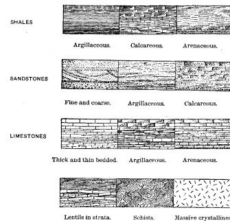
Fig. 2. Symbols used to represent different kinds of rocks.
