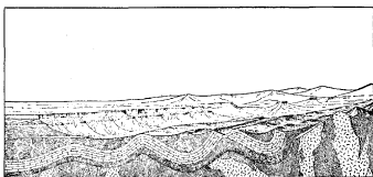
Fig. 3. Showing a vertical section in the front of the picture, with a landscape above.
