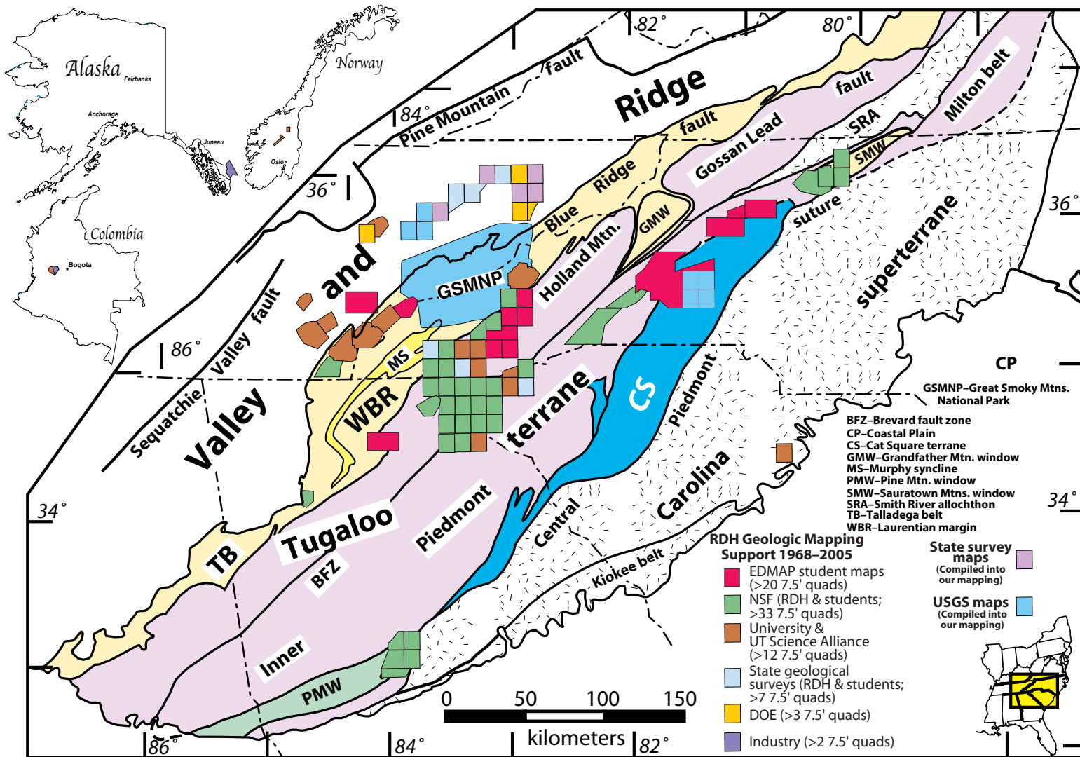
Southern Appalachians base map modified from Hatcher et al., 1990, Tectonic Map of the US Appalachians, Geological Society of America, Geology of North America, v. F2, Plate 1.
