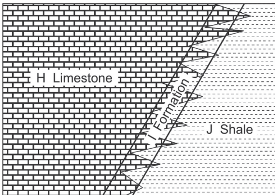
C.--Possible boundaries for a laterally intertonguing sequence
