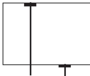
D.--Interval Biozone (based on highest occurrences).
