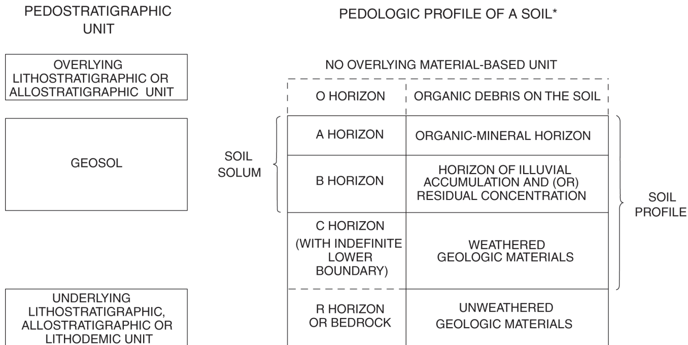
TEXT-FIGURE 6 Relation between pedostratigraphic units and pedologic profiles. The base of a geosol is the lowest clearly defined physical boundary of a pedologic horizon in a buried soil profile. In this example, it is the lower boundary of the B horizon because the base of the C horizon is not a clearly defined physical boundary. In other profiles, the base may be the lower boundary of a C horizon. Pedologic profile modified from Ruhe (1965) and Pawluk (1978).
