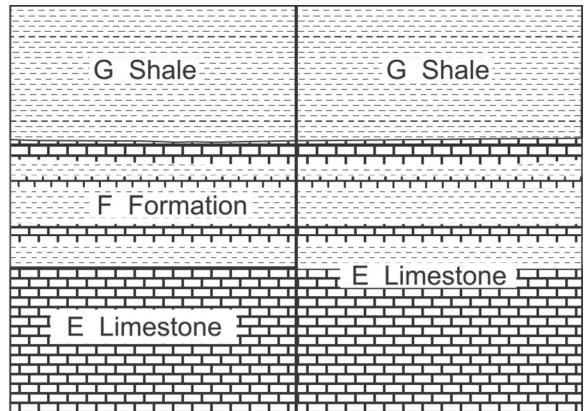
B.--Alternative boundaries in vertically gradational or interlayered sequence
