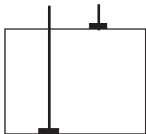
C.--Interval Biozone (based on lowest occurrences).
