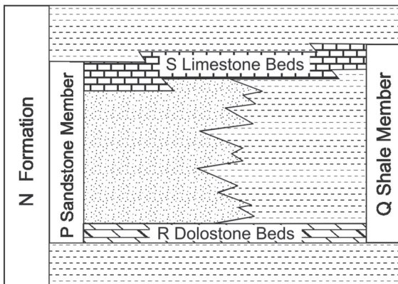
E.--Key beds, here designated the R Dolostone Beds and the S Limestone Beds, are used as boundaries to distinguish the Q Shale Member from other parts of the N Formation. A lateral change in composition between the key beds requires that another name, P Sandstone Member, be applied. The key beds are part of each member
