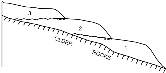
TEXT-FIGURE 8 Example of allostratigraphic classification of contiguous deposits of similar lithology. Allostratigraphic units 1, 2, and 3 are physical records of three glaciations. They are lithologically similar, reflecting derivation from the same bedrock, and constitute a single lithostratigraphic unit.
