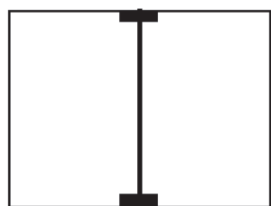
A.--Taxon-range Biozone (based the range of a taxon).
