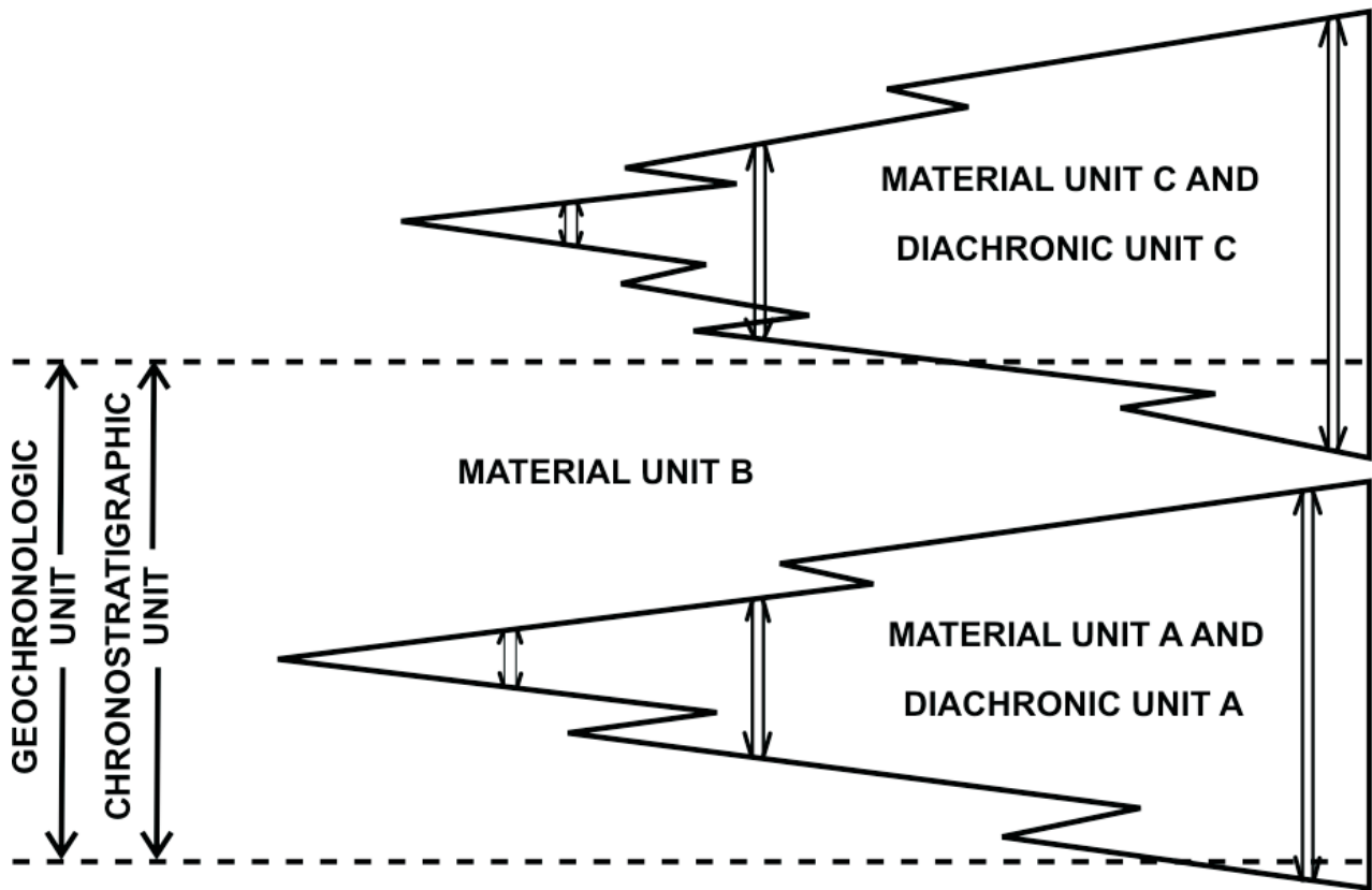
TEXT-FIGURE 10 Comparison of geochronologic, chronostratigraphic, and diachronic units.
